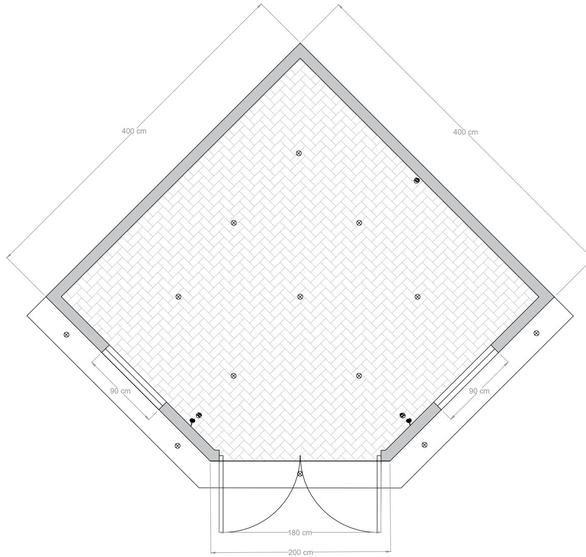
Outbuilding 16 Sqm Type01
