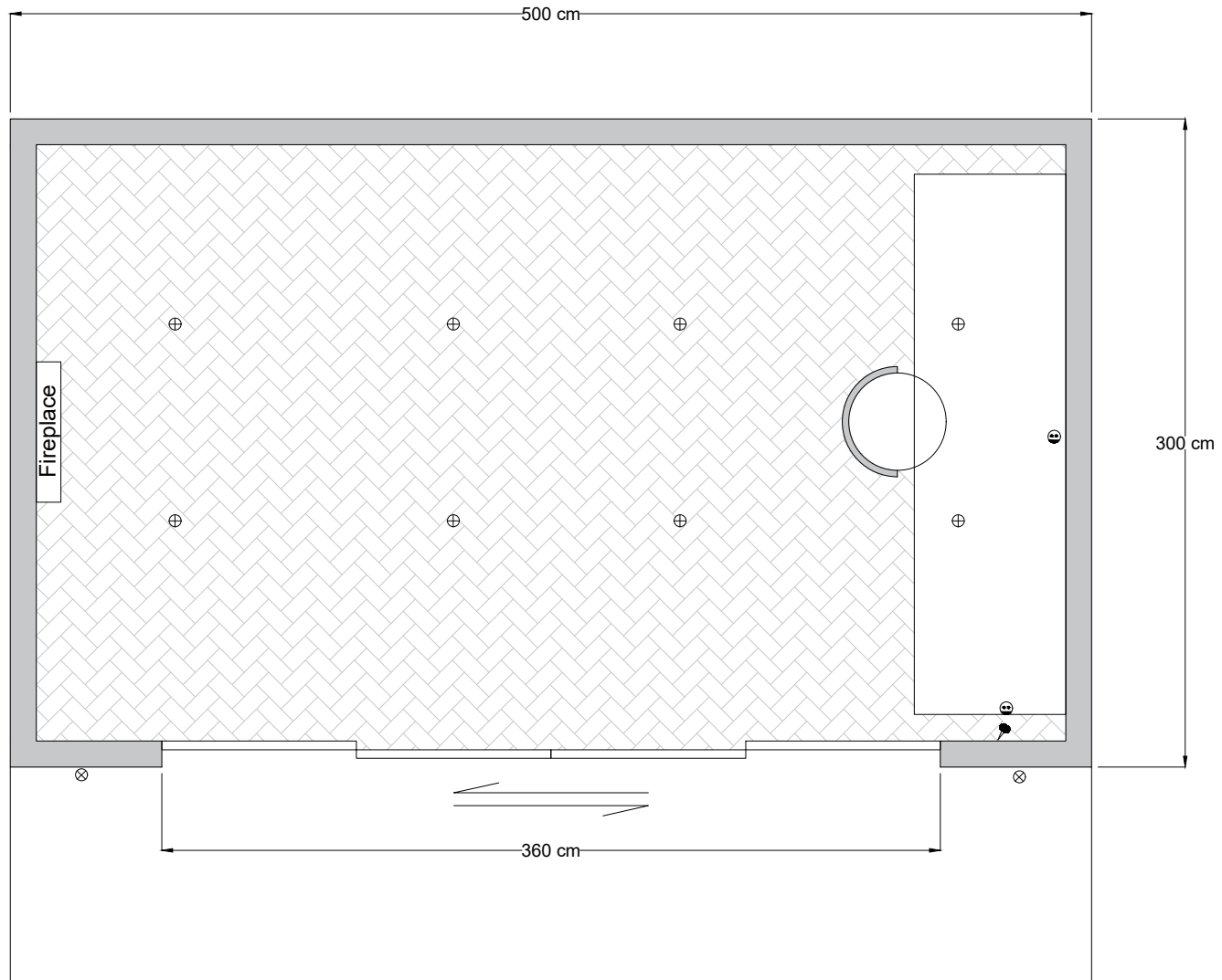
Outbuilding 15 Sqm Type02
