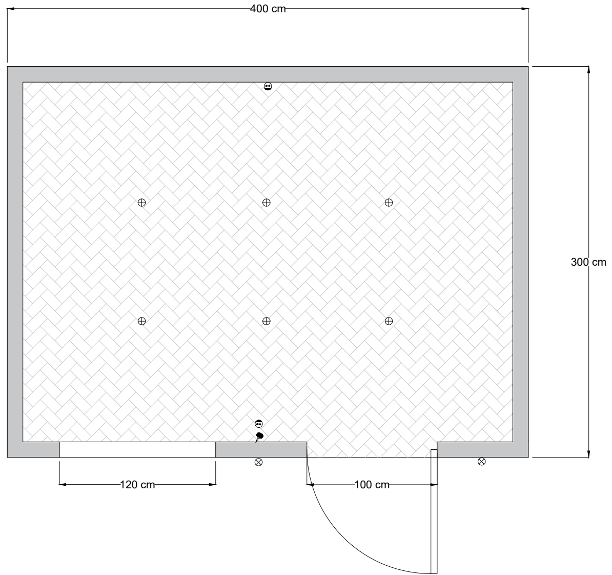
Outbuilding 12 Sqm Type05
