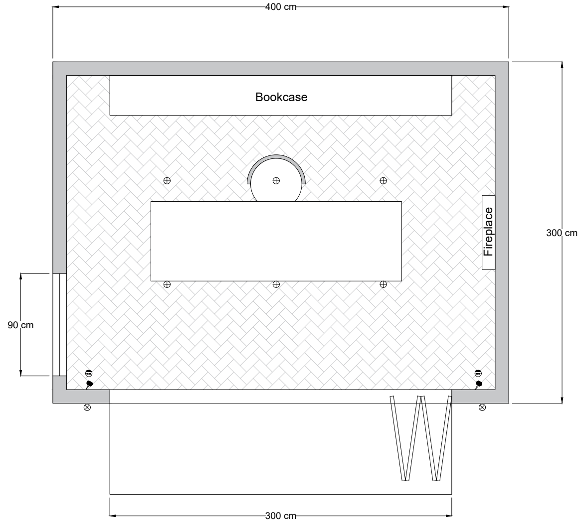
Outbuilding 12 Sqm Type03
