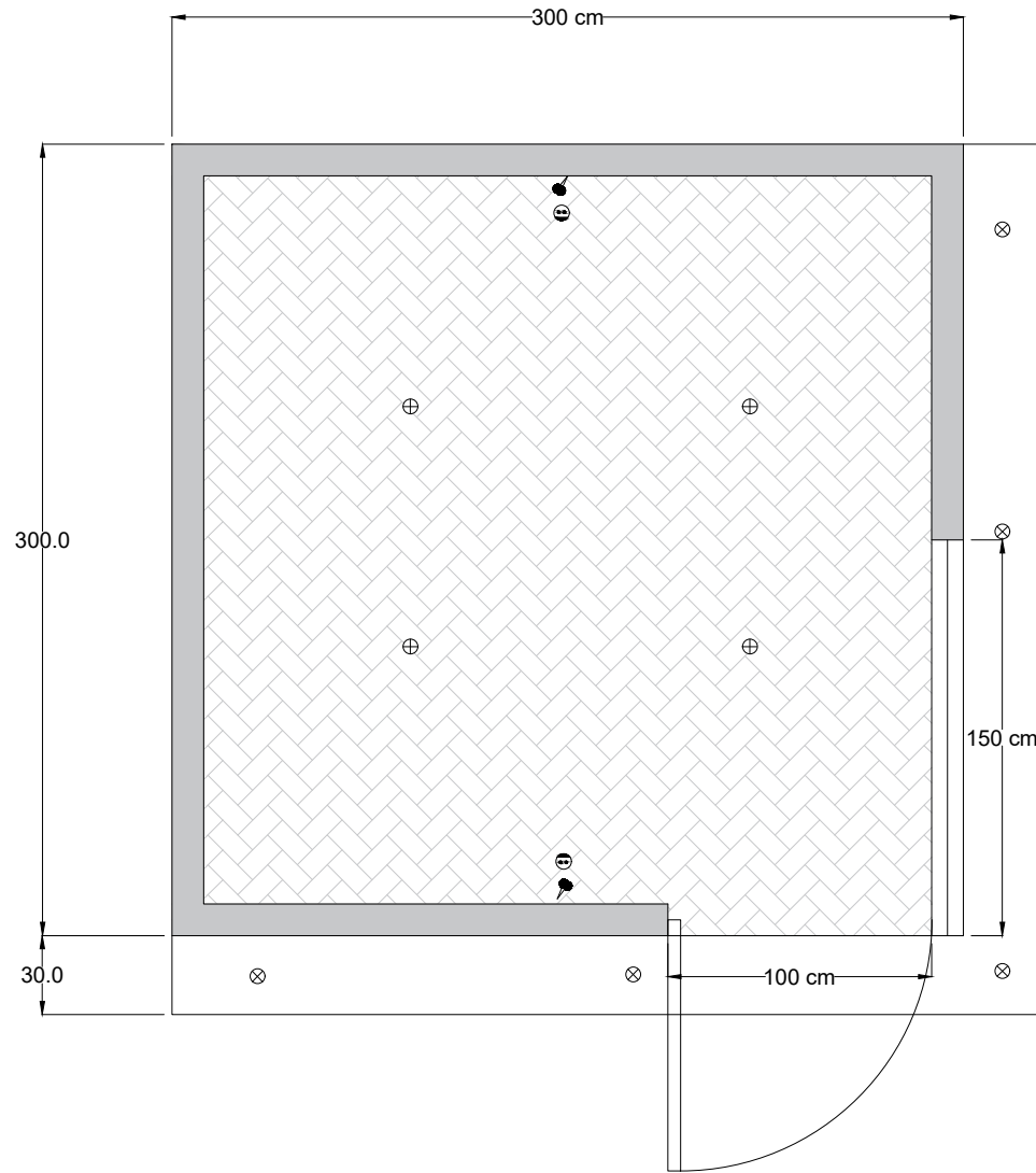
Outbuilding 9 Sqm Type06
