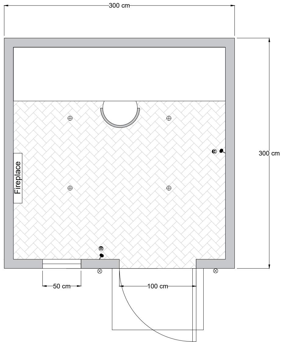
Outbuilding 9 Sqm Type02
