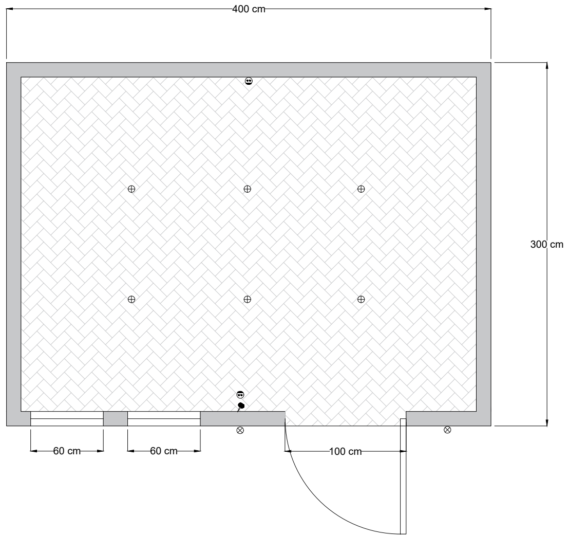
Outbuilding 12 Sqm Type05
