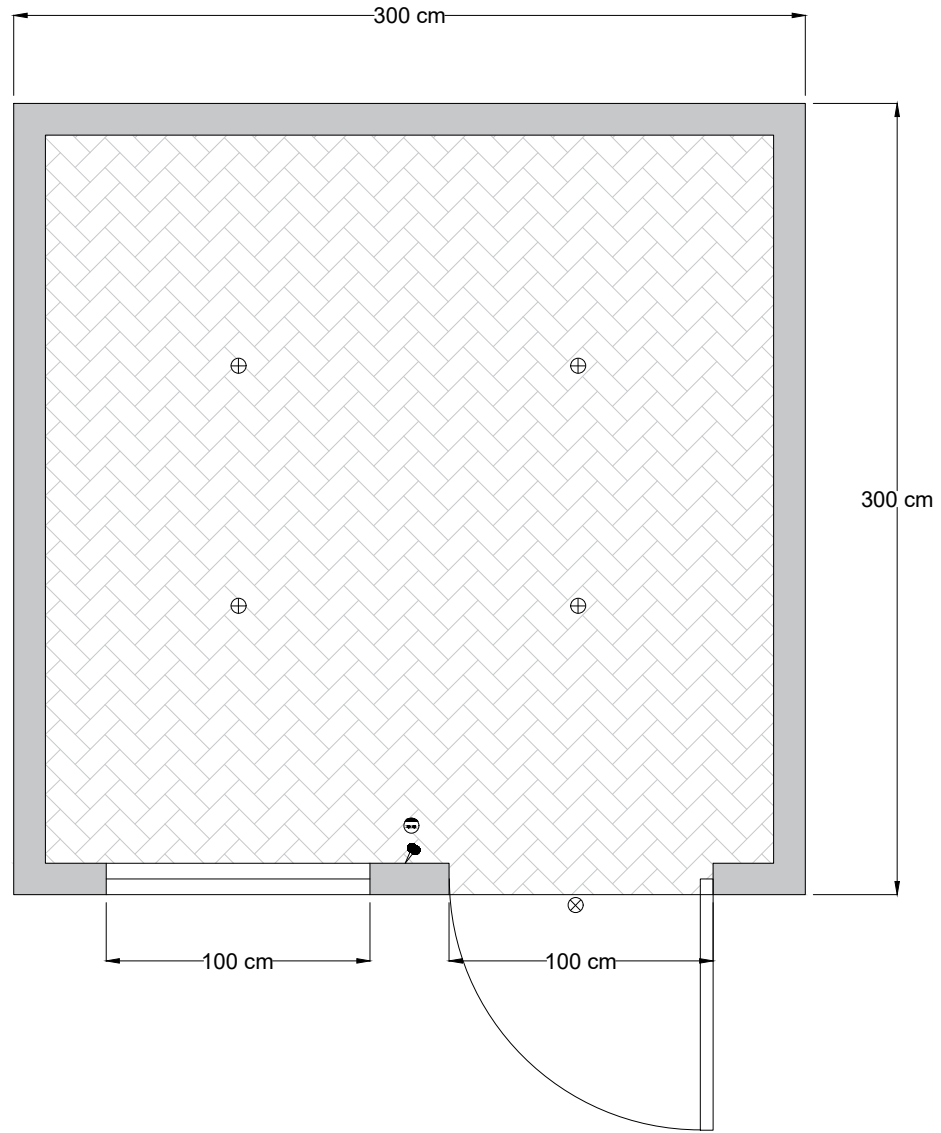
Outbuilding 9 Sqm Type05
