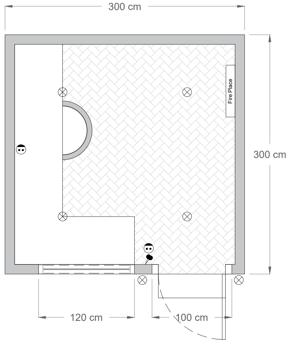
Outbuilding 9 Sqm Type01
